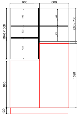
SOPRACOLONNA "MATRIX" PER COLONNE H 96/132 ZOCCOLO H 13 SENZA GOLA "MATRIX" OVER COLUMN PANEL FOR COLUMNS H 96/132 PLINTH H 13 WITHOUT FINGER RAIL
