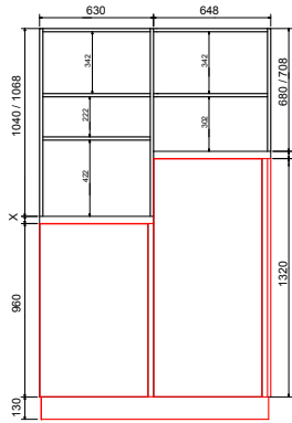
SOPRACOLONNA "MATRIX" PER COLONNE H 96/132 ZOCCOLO H 13 SENZA GOLA "MATRIX" OVER COLUMN PANEL FOR COLUMNS H 96/132 PLINTH H 13 WITHOUT FINGER RAIL
